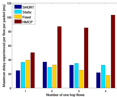
Fig. 18. Maximum delays for multiple one hop flows from a node
