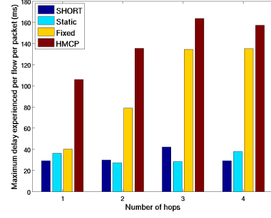
Fig. 7. Maximum delay for unidirectional flows
