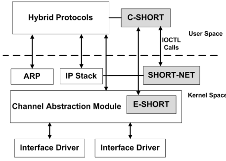
Fig. 5. System architecture with SHORT-specific components in gray
