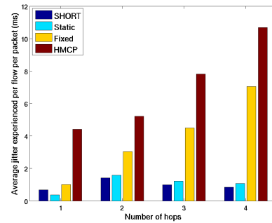
Fig. 10. Average jitter for bidirectional flows
