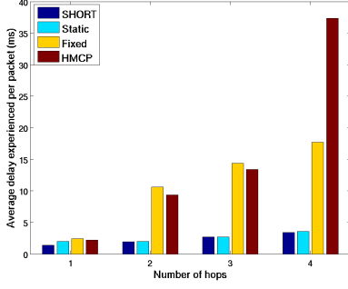
Fig. 6. Average delay for unidirectional flows
