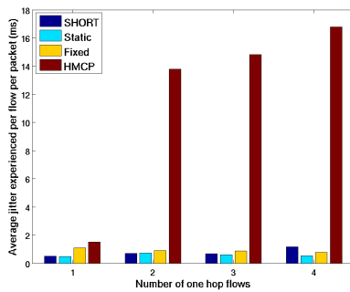
Fig. 19. Average jitter for multiple one hop flows from a node
