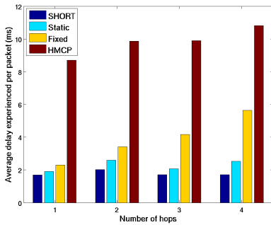
Fig. 13. Average delay of VoIP packets sent with a UDP flow
