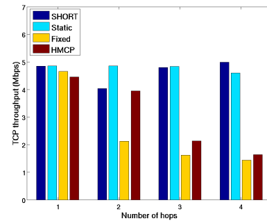
Fig. 16. Throughput of TCP flow went with a VoIP flow
