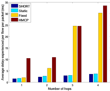
Fig. 11. Average delay for bidirectional flows
