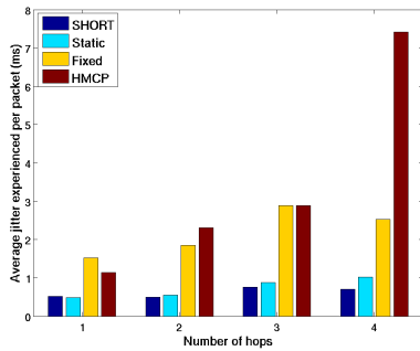
Fig. 9. Average jitter for unidirectional flows
