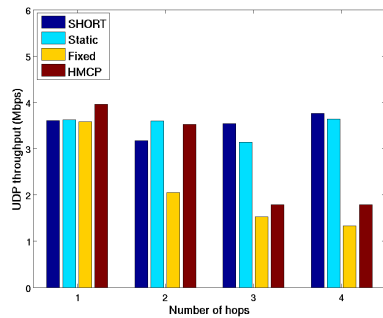
Fig. 15. Throughput of UDP flow went with a VoIP flow
