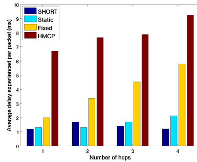
Fig. 14. Average delay of VoIP packets sent with a TCP flow
