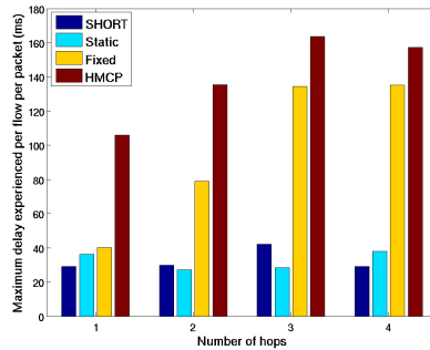
Fig. 12. Maximum delay for bidirectional flows
