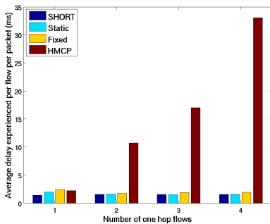
Fig. 17. Average delays for multiple one hop flows from a node
