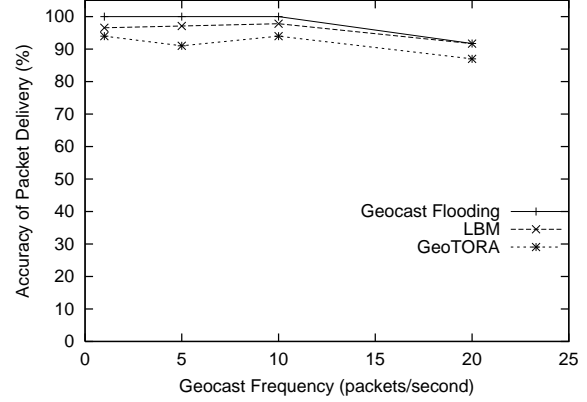
Figure 12. Accuracy of Delivery versus Geocast Frequency
