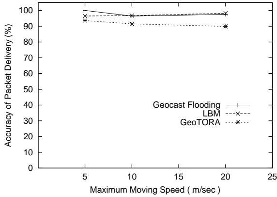
Figure 10. Accuracy of Delivery versus Speed
