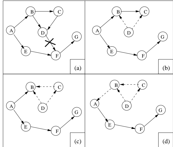
Figure 1. Route Maintenance in TORA: Route maintenance is required due to failure of the link between nodes D and F. In the figure, a link that has been reversed since the initial state is shown as a dashed line.
