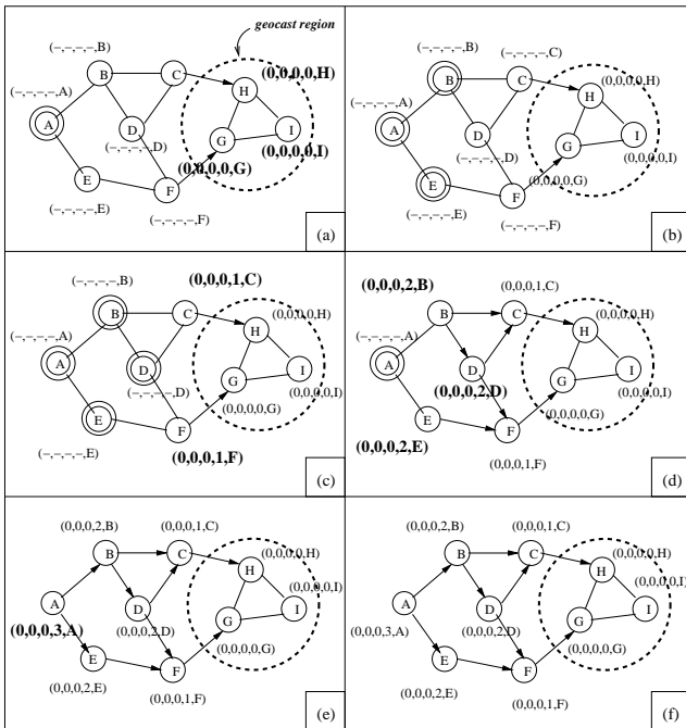
Figure 5. Geocast Route Creation in GeoTORA
