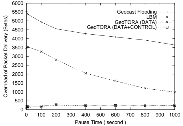
(b) Overhead of Geocast Delivery (Bytes)
