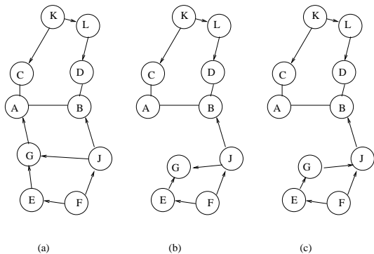
Figure 2. Anycasting using modified TORA
