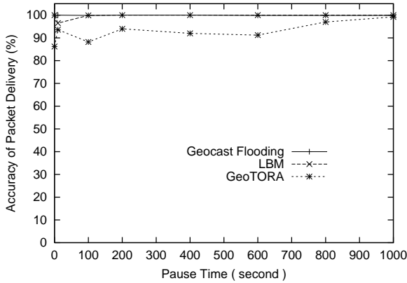
Figure 8. Accuracy of Delivery versus Pause Time
