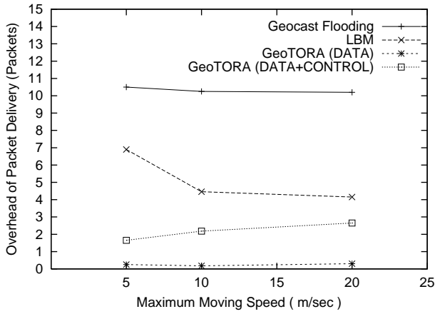
(a) Overhead of Geocast Delivery (Packets)
