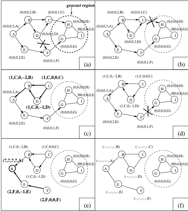
Figure 6. Geocast Route Maintenance in GeoTORA: Three different scenarios of link failure
