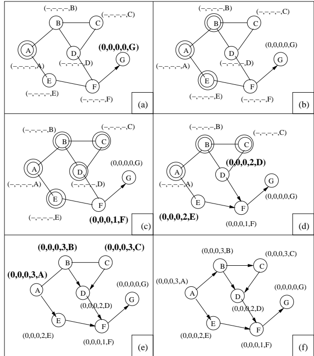
Figure 4. Route Creation Phase in TORA: In the figure, a circle around a node indicates that the route-required flag is set. Arrows on each wireless link points from the higher height node to the lower height node. The height is depicted as a 5-tuple, as explained in the context.
