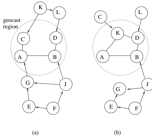
Figure 3: Geocasting using GeoTORA
