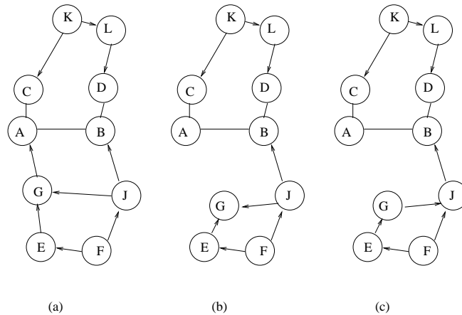
Figure 2: Anycasting using modified TORA
